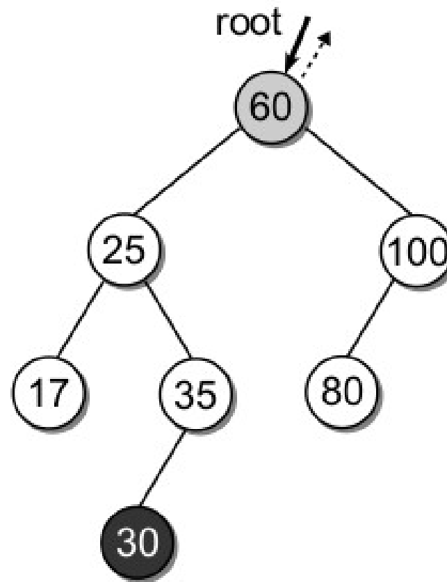
(i) root = bstInsert(...)
