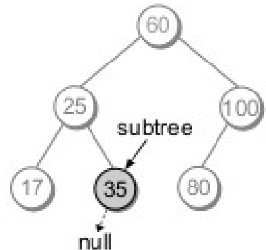
(c) bstInsert(subtree.right, key)
