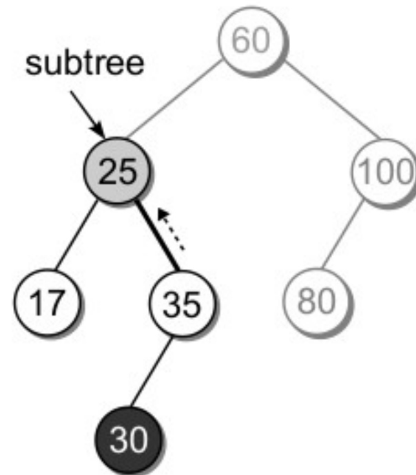
(g) subtree.right = bstInsert(...)
