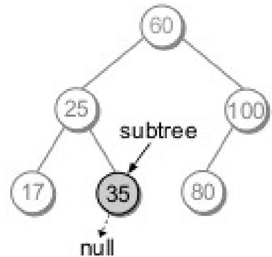
(c) bstInsert(subtree.right, key)
